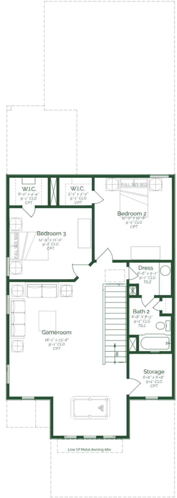
SECOND FLOOR
