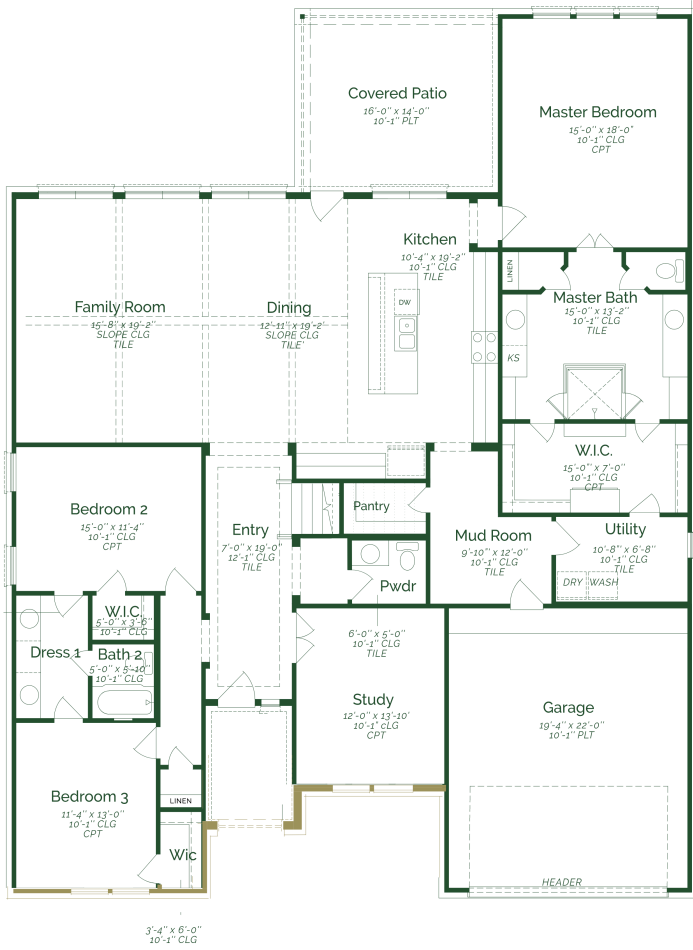
Floor 1
